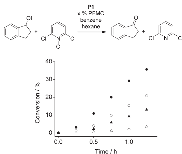
Figure 1. Oxidation of 1-indanol by \text{Cl}_2\text{pyNO} with the polymeric catalyst P1 in solvents containing various amounts of PFMC ( \Delta : 0 %; \blacktriangle : 10 %; \circ : 20 %; \bullet : 40 %). The reactions were performed in mixtures of benzene, hexane and PFMC at 55^\circ\text{C} with a substrate/ \text{Cl}_2\text{pyNO} /catalyst molar ratio of 100:100:1. The data points represent averaged values from two independent experiments.
