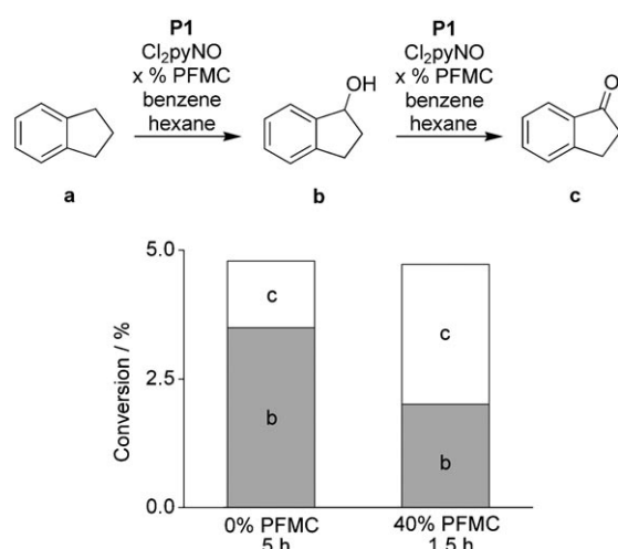
Figure 2. Oxidation of indane by \text{Cl}_2\text{pyNO} with the polymeric catalyst P1 in solvents containing 0% or 40% of PFMC. The reactions were performed in mixtures of benzene, hexane and PFMC at 55^\circ\text{C} with a substrate/ \text{Cl}_2\text{pyNO} /catalyst molar ratio of 100:200:1. The data represent averaged values from two independent experiments.
